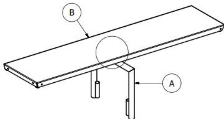
DETALLE UNION TABLON A BASE
